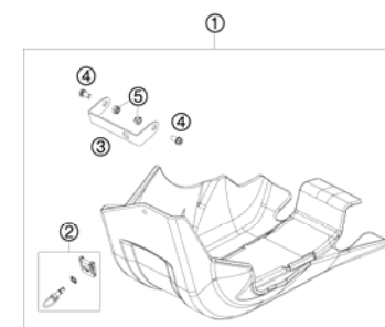
ENGINE GUARD
