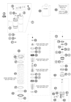
SHOCK ABSORBER DISASSEMBLED
