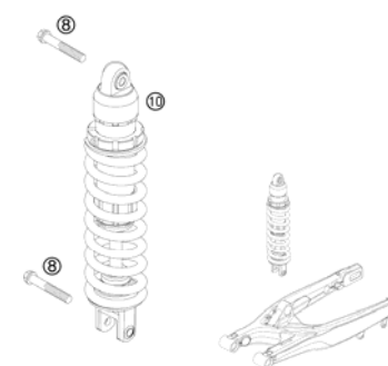
SHOCK ABSORBER
