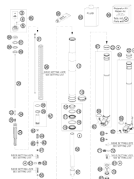
FRONT FORK DISASSEMBLED
