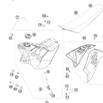
TANK, SEAT, COVER
