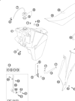
TANK, SEAT, COVER
