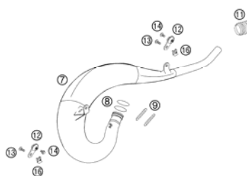
EXHAUST PIPE
