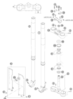
FRONT FORK WP USD 48
