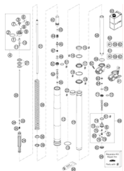
FORK LEGS WP USD 48
