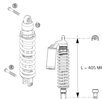
MONOSHOCK WP
