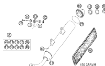
EXHAUST SILENCER
