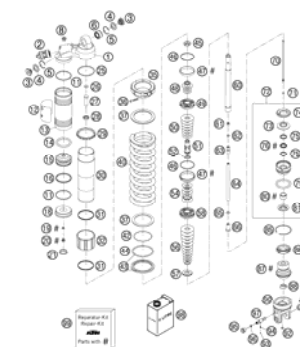
MONOSHOCK DISASSEMBLED
