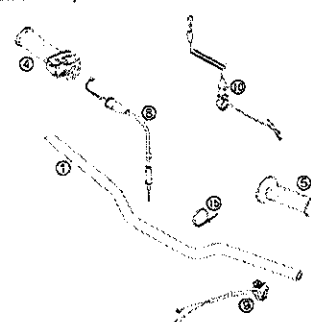
LENKER, ARMATUREN HANDLEBAR, CONTROLS
