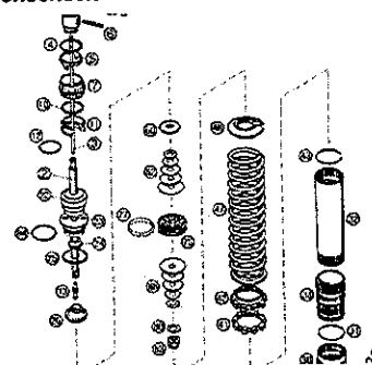
FEDERBEIN ZERLEGT JUNIOR LC MONOSHOCK DISASSEMBLED JUNIOR LC
