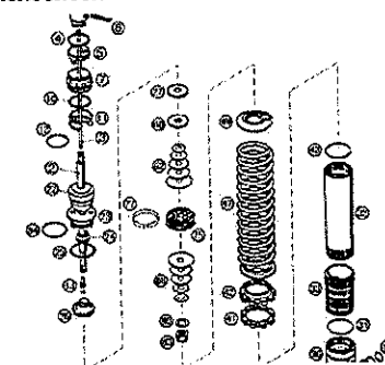
FEDERBEIN ZERLEGT SENIOR LC MONOSHOCK DISASSEMBLED SENIOR LC
