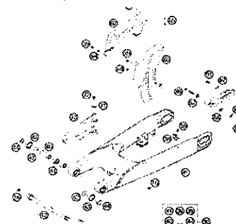
SCHWINGARM, KETTENSCHUTZ SWING ARM, CHAIN GUARD
