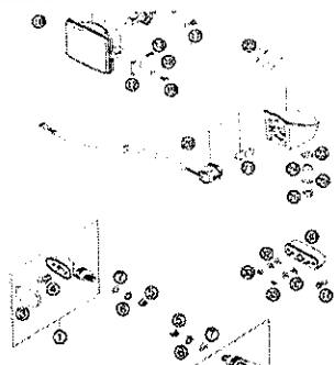
LICHTANLAGE LIGHTING SYSTEM
