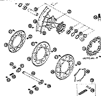
HINTERRAD 18" REAR WHEEL 18"
