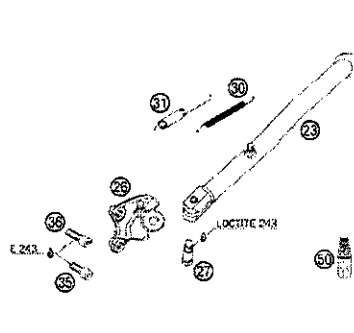
FEDERBEIN WP MONOSHOCK WP
