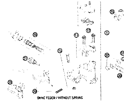
PRO LEVER ANLENKUNG PRO LEVER SYSTEM
