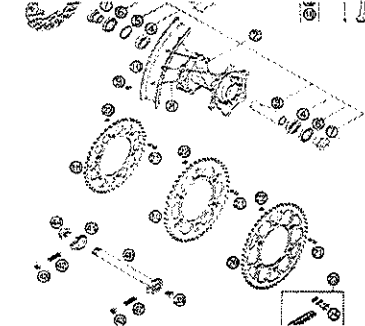
HINTERRAD 18" + 19" REAR WHEEL 18" + 19"
