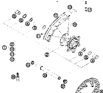
VORDERRAD 21" FRONT WHEEL 21"
